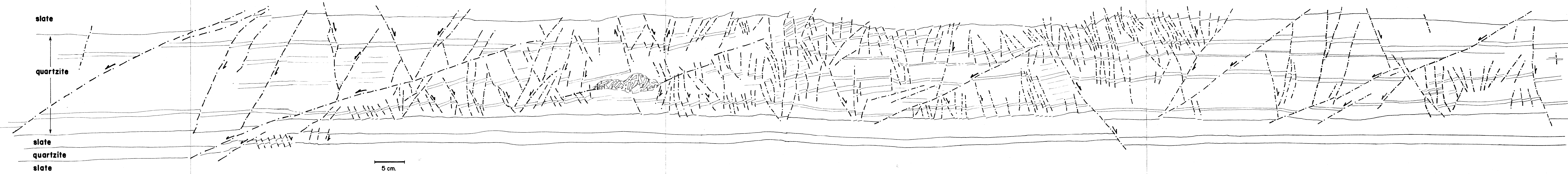
PLATE 9 SHEAR FRACTURE PATTERN IN THICKER QUARTZITE UNIT, YORK CLIFFS LAYER-PARALLEL SINISTRAL BRITTLE SHEAR STRUCTURE (SCALE 1:2)
