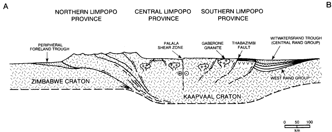
Fig. 13. Cross section through the Kaapvaal and Zimbabwe Cratons across the Limpopo Province, a product of the collision between the two cratons at approximately 2.7 Ga ago. It is suggested in this diagram that the upper Witwatersrand strata were deposited in a foreland basin on the cratonward side of an uplifted plateau overlying continent greatly thickened (similar to Tibet) in the Kaapvaal/Zimbabwe collision.
