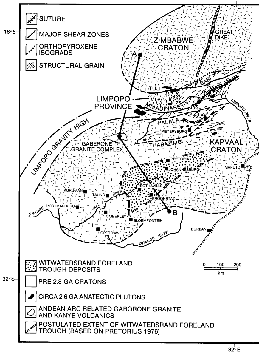
Fig. 10. Map showing the location of the Witwatersrand Trough in relation to the Limpopo continental collision zone, the Gaborone Granite Complex, and numerous shear zones attributed to uplift and sideways motion of the region to the north of the Witwatersrand Basin. Anatectic granites (in black) are related to the collision between the Kaapvaal and Zimbabwe Cratons. The less intensely ornamented basement marks the future site of Ventersdorp rifting. Map based on data compiled from Tankard et al. [1982]; Visser et al. [1976]; Pretorius, [1976]; and Button [1981].
