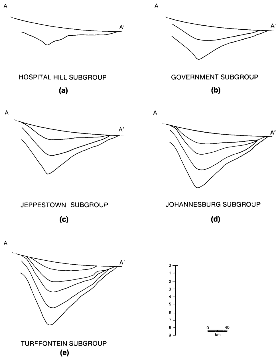
Fig. 6. Cross section showing shape of sediment wedge in Witwatersrand Basin determined from isopachs: (a) Hospital Hill Subgroup; (b) after deposition of Government Subgroup; (c) after deposition of Jeppestown Subgroup; (d) after deposition of Johannesburg Subgroup; (e) after deposition of Turffontein Subgroup. Note the asymmetry and complexity at the southern end of the sections.
