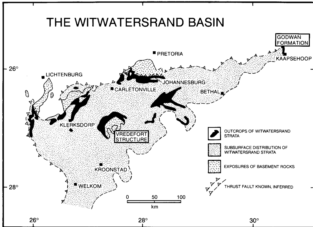
Fig. 3. Map of the Witwatersrand Basin showing locations referred to in text, outcrop and subsurface distribution of Witwatersrand strata, locations of exposed basement, and the generally fault-bounded northwestern basin margin (map compiled from Pretorius [1976] and Button [1977]).
