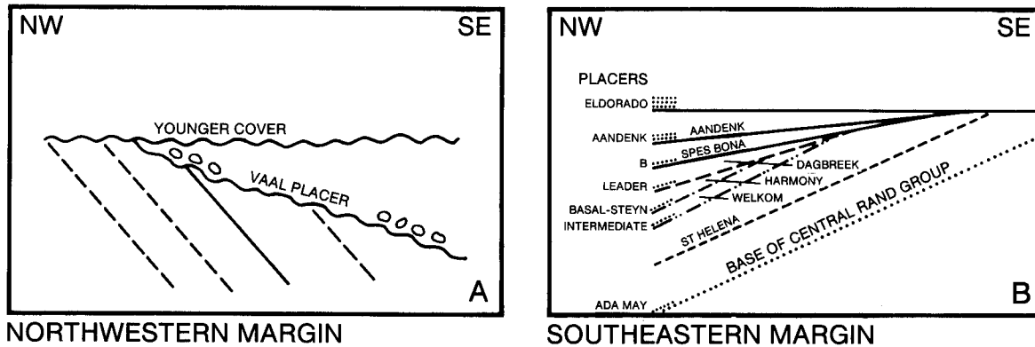
Fig. 9. Schematic vertical cross-sections of upper Witwatersrand strata from near the (a) northwestern and (b) southeastern basin margins. Section 9b is from Tankard et al. [1982].
