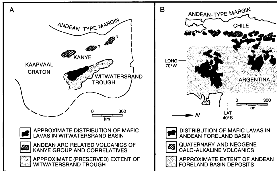
Fig. 12. Comparison of areas of mafic lava flows in the Witwatersrand Basin (Crown and Bird lavas) with distribution of mafic lava flows in the Andean foreland basin of the southern Andes (map 12b modified from Reunion de la Carte Geologique de L'Amerique du Sud [1968]).
