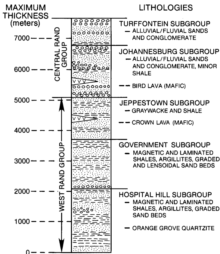
Fig.2. Generalized stratigraphic column for the Witwatersrand Supergroup. The quoted thicknesses are maximum values which are found near the northwestern basin margin, while the strata thin towards the southeastern basin margin.
