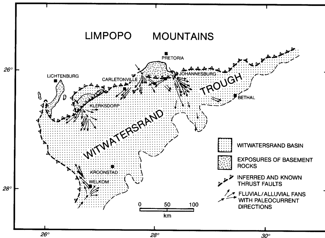
Fig. 7. Paleocurrent directions derived from upper Witwatersrand strata showing that sediments of the Central Rand Group largely prograded into the basin from the northwestern margin in the form of alluvial and fluvial fans. Some transport of sediments into the basin from its southwestern margin is indicated by paleocurrents from Welkom, and some along axis transport has also been noted from sediments between Kroonstad and Klerksdorp. Paleocurrent directions are from Brock and Pretorius [1964].
