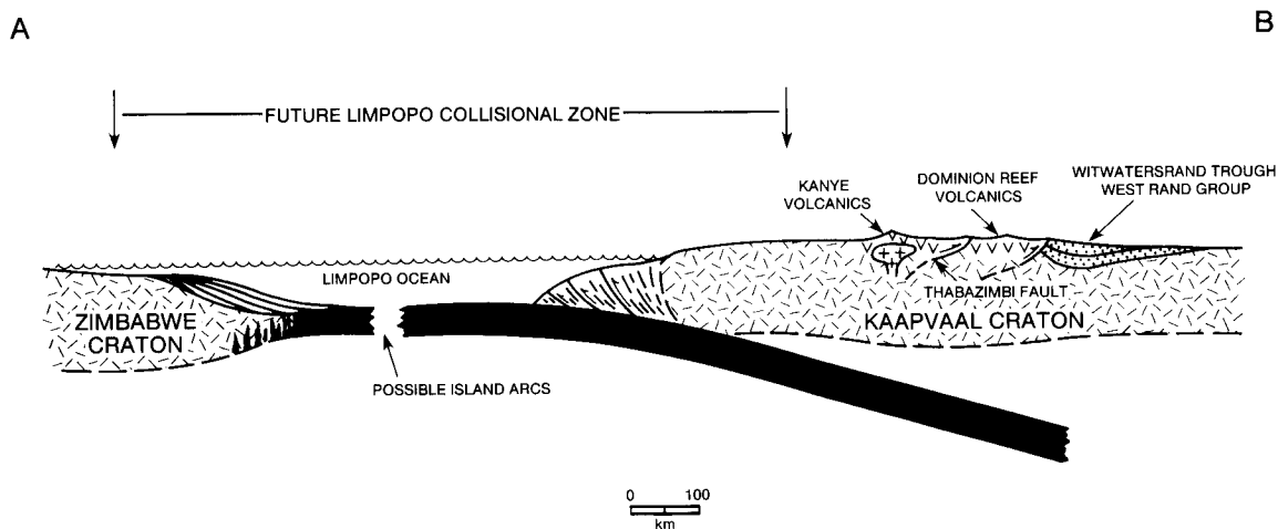
Fig. 11. Tectonic elements suggested for the Kaapvaal and Zimbabwe Cratons during deposition of the lower Witwatersrand Supergroup. The present northern margin of the Kaapvaal Craton includes an Archean Andean margin; the volcanic arc is represented by the Kanye Volcanics, the Dominion Volcanics, and lateral equivalents. Rocks of the Witwatersrand Supergroup (West Rand Group) were deposited in a foreland basin bound on the north by an active fold and thrust belt. All rocks within the "future Limpopo collisional zone" became highly deformed and metamorphosed when the Kaapvaal and Zimbabwe Cratons collided approximately 2.7 Ga ago.
