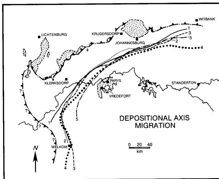
Fig. 8. Location of the depositional axis of the Witwatersrand Basin during (1) Hospital Hill, (2) Government, (3) Jeppestown, (4) Johannesburg, and (5) Turffontein times. This axis generally, but not universally, migrated toward the southeast during deposition of the Witwatersrand strata, possibly suggesting an interplay of elastic flexure of the lithosphere, elasticoviscous relaxation, and sedimentary progradation.
