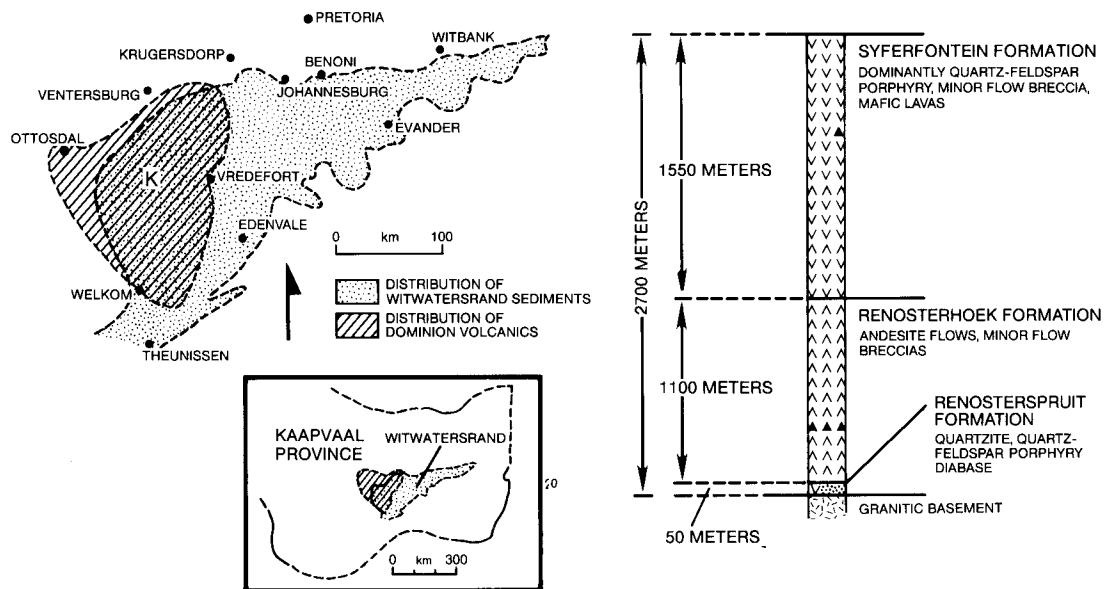
Fig. 4. Distribution, thickness, and lithologies in the largely volcanic Dominion Group [after SACS., 1980; Tankard et al., 1982]. Symbol K shows the location of Klerksdorp.
