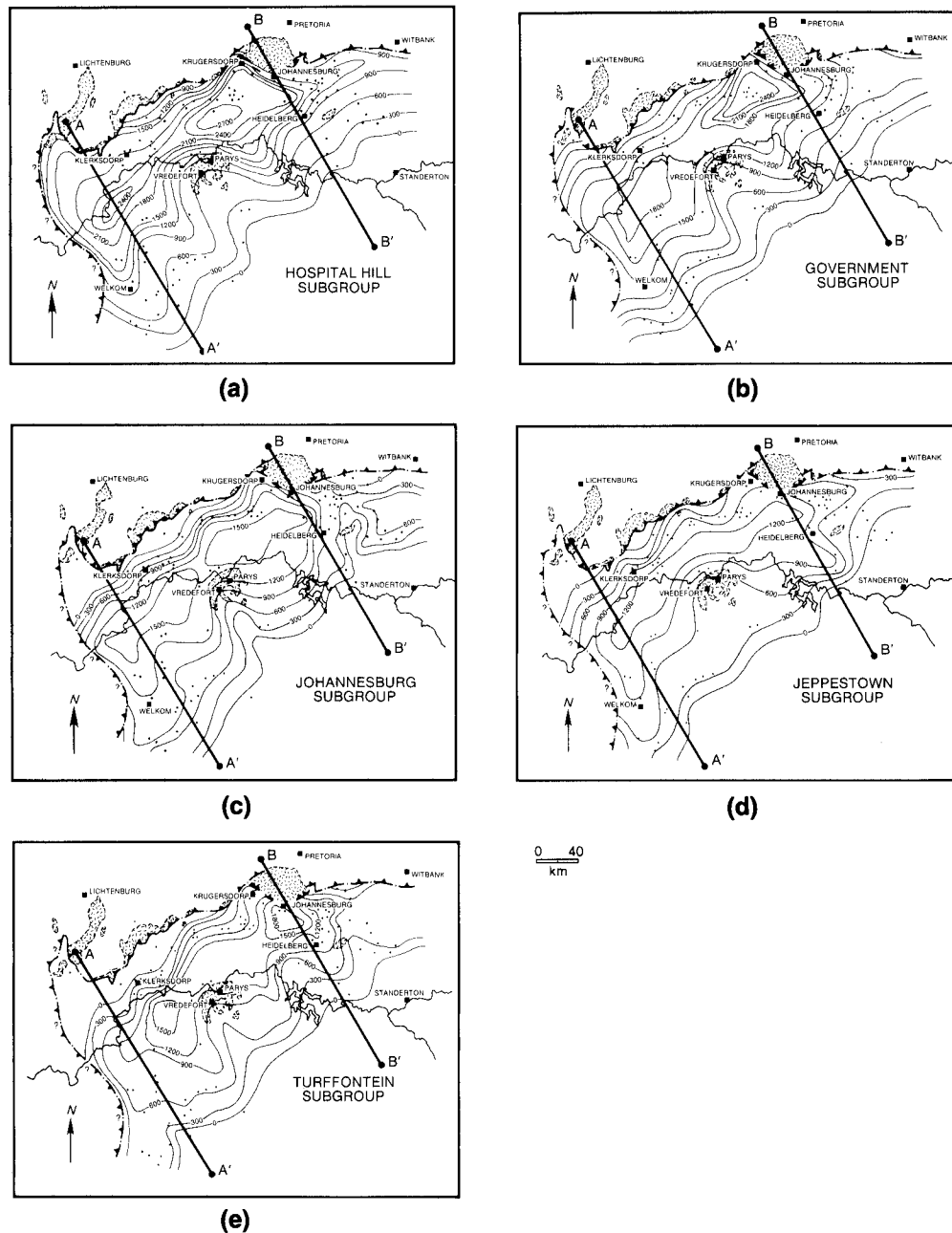
Fig. 5. Isopach maps of the Witwatersrand Basin showing the thickness (in meters) and distribution: (a) Hospital Hill Subgroup; (b) Government Subgroup; (c) Johannesburg Subgroup; (d) Jeppestown Subgroup; (e) Turffontein Subgroup. Figures redrawn after Brock and Pretorius [1964]. The basin is strikingly similar to foreland troughs both in width (220 km) and in asymmetry. Copies of cross sections B-B' are not published but are available from Burke at LPI.
