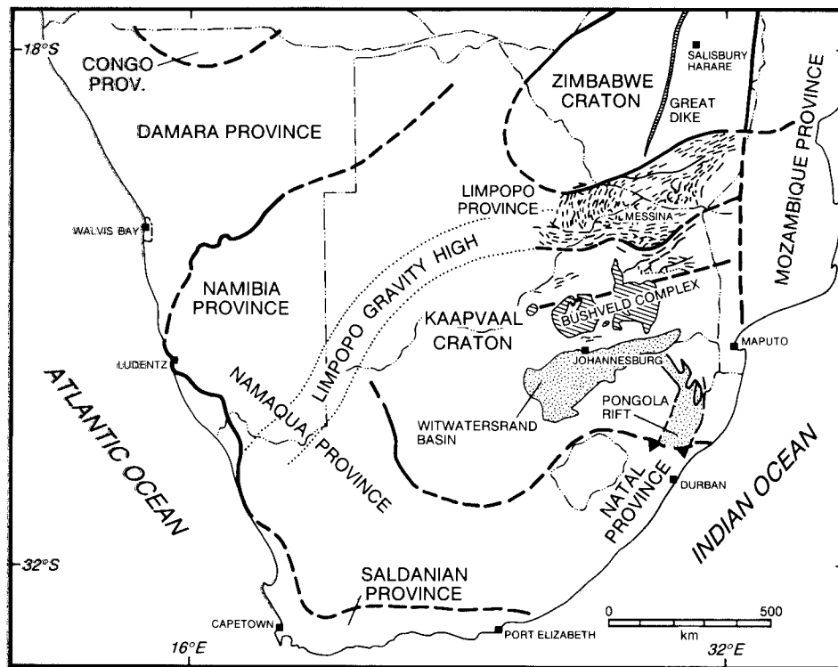
Fig. 1. Generalized map of southern Africa showing the location of the Witwatersrand Basin on the Kaapvaal Craton, as well as the distribution of other selected Precambrian geologic elements. Note that the Witwatersrand Basin is elongated parallel to, but located some distance south of the high-grade Limpopo Province (map modified after Tankard et al. [1982]).
