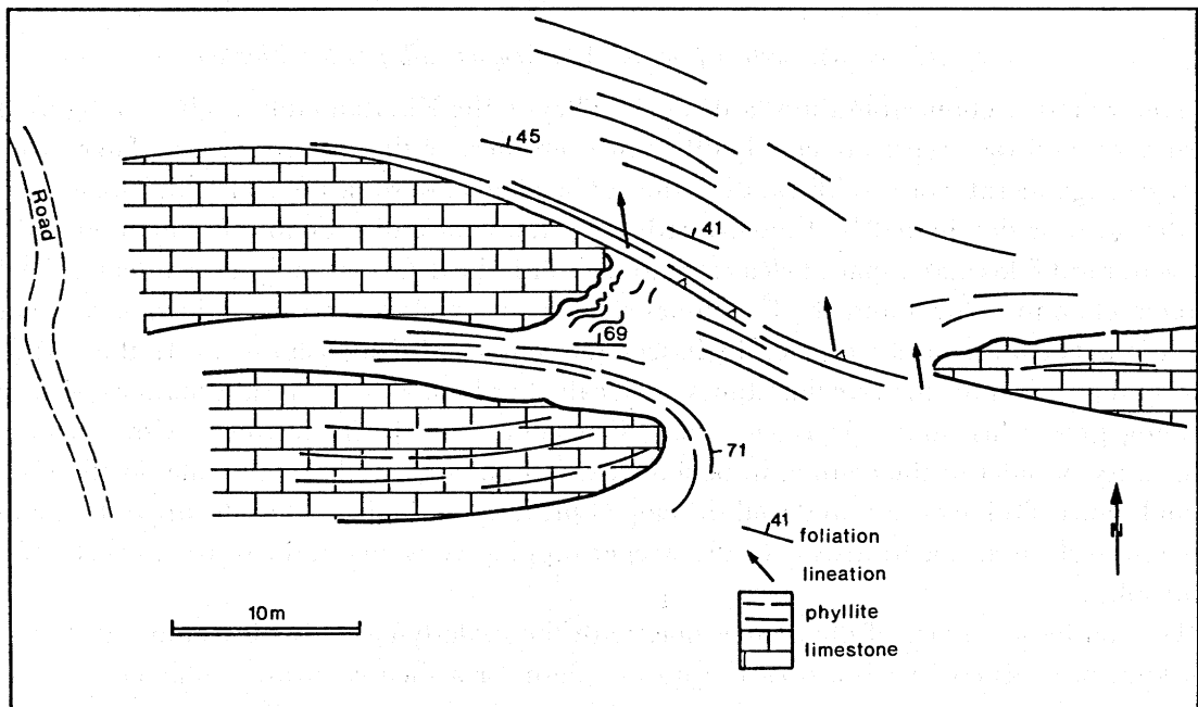
FIGURE 4. Sketch map of locality S471 on the eastern Kunlun section, to show the shear deformation breaking the structure to give a tectonic melange.
