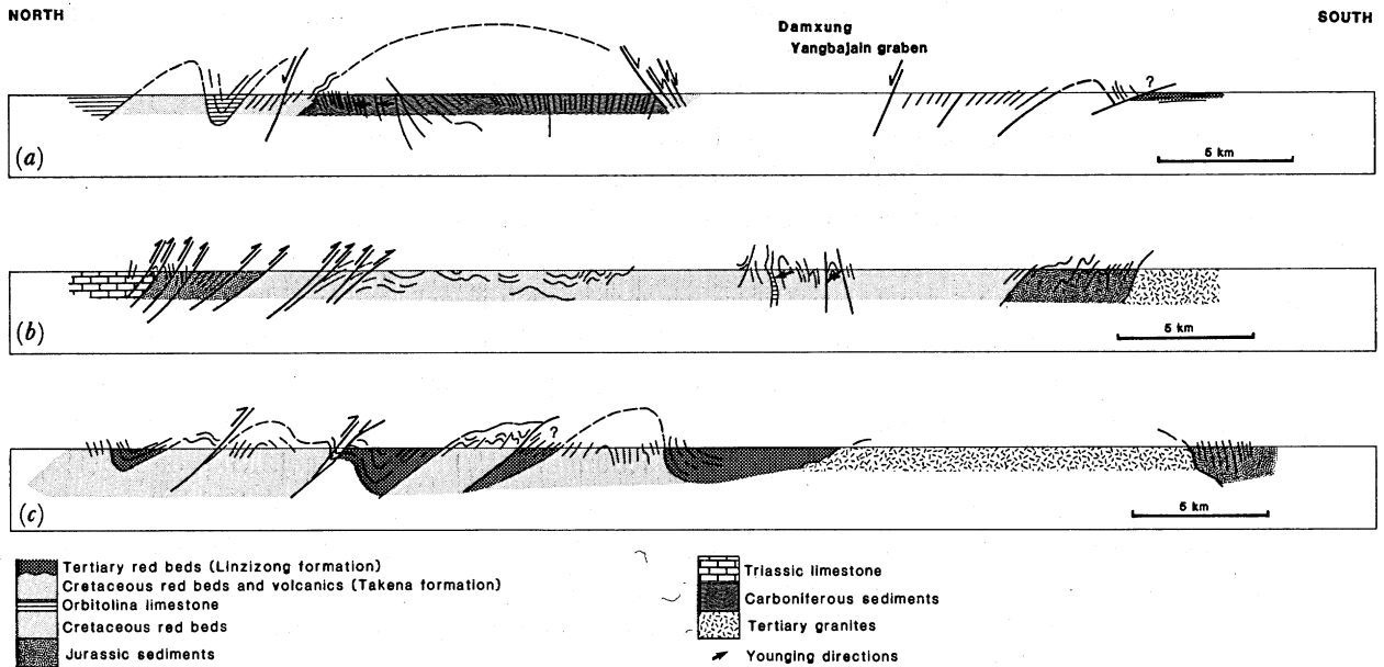
FIGURE 9. Cross sections through the southern part of the Lhasa Terrane, from the Nam Co to north of Lhasa; lines are shown on figure 1. The '?' indicate a degree of uncertainty in the age and/or structure of the red beds.
