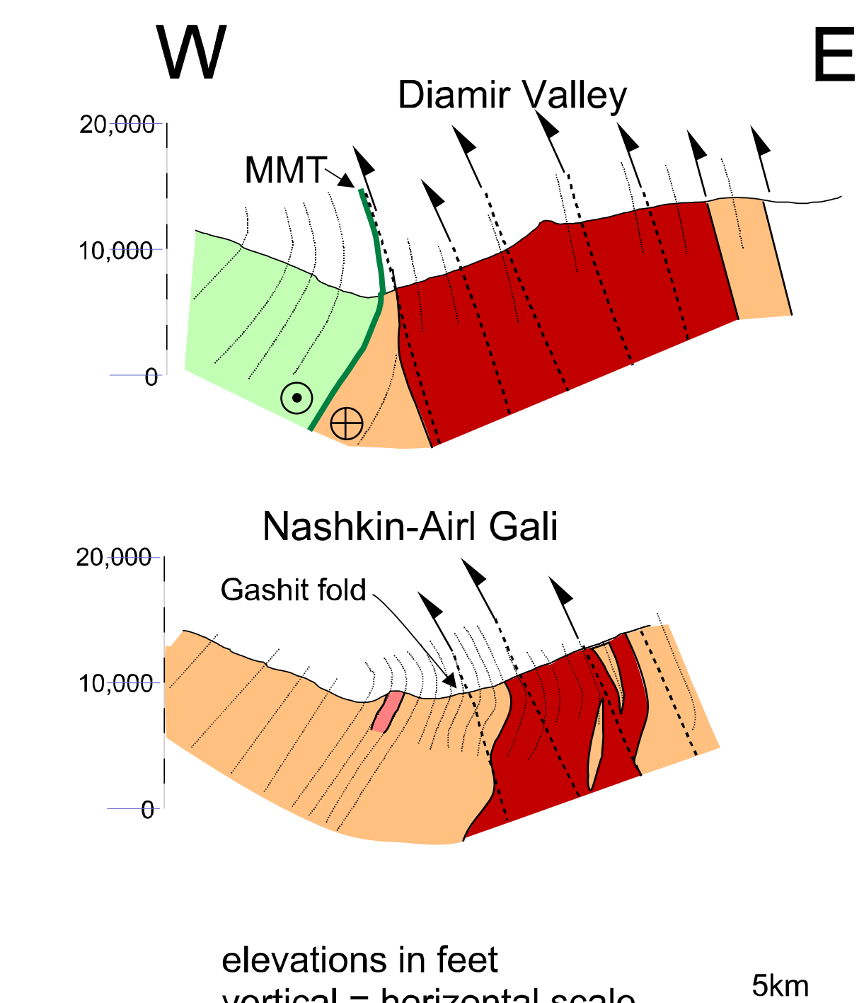
Fig 3 - Cross sections of the southwestern margin of the Nanga Parbat structure
