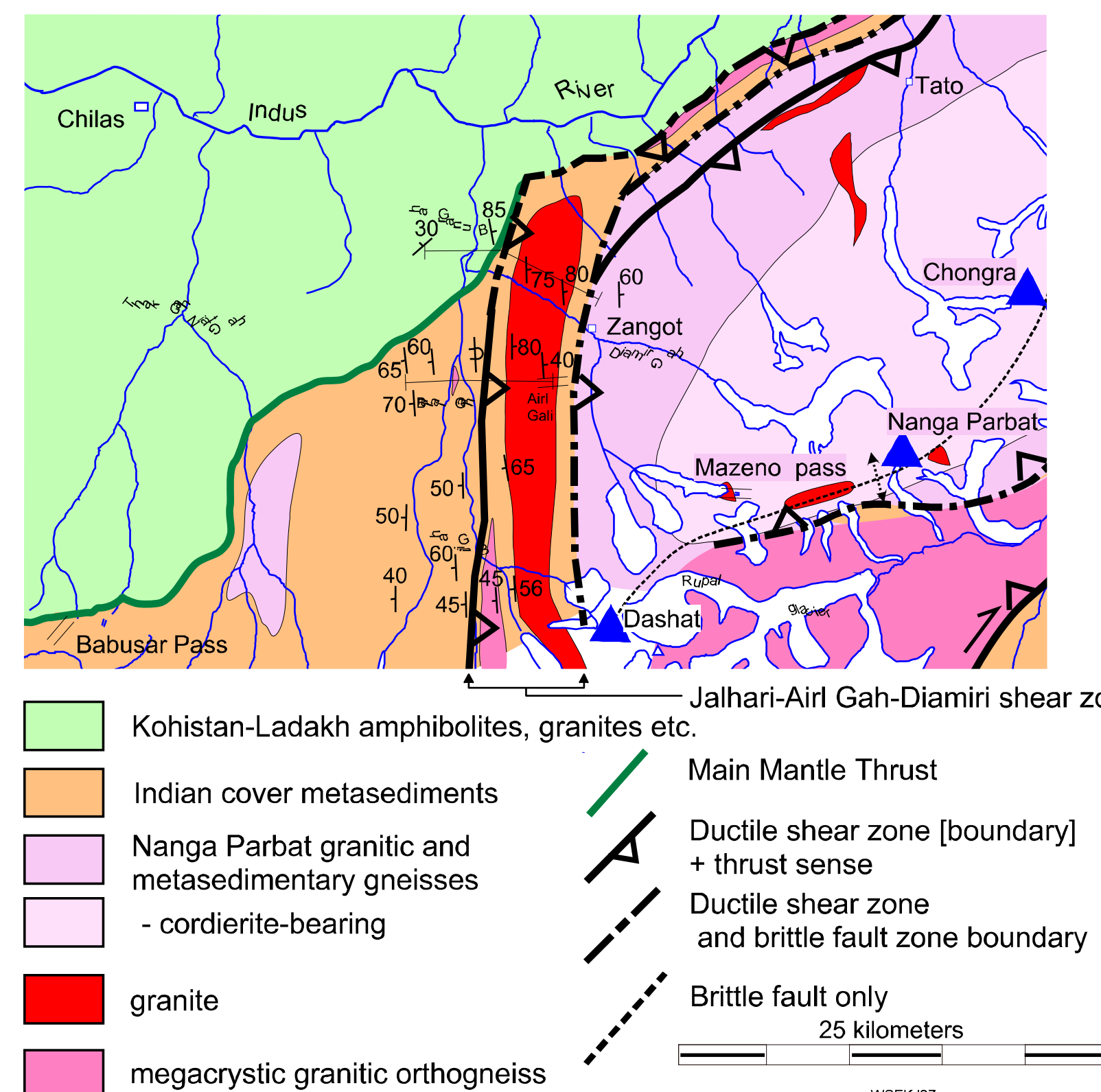
Fig. 2a Southwest Nanga Parbat Massif
