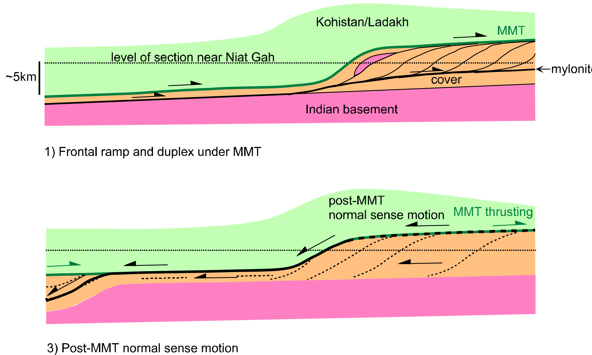
Fig. 5 Cartoon structure sections prior to Nanga Parbat massif uplift and exhumation
