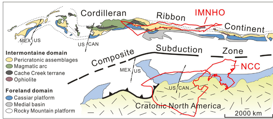
Fig. 21. Map of Cordilleran Ribbon Continent before it accreted to North America, forming large segments of the present North American Cordilleran Orogen. Modified from Johnston (2008). Red outlines show the southern NCC reconstructed before the proposed collision with the composite Yinshan Ribbon Microcontinent, arc, and accretionary orogen in the IMNHO, overlain on the pre-collision North American Cordillera.
