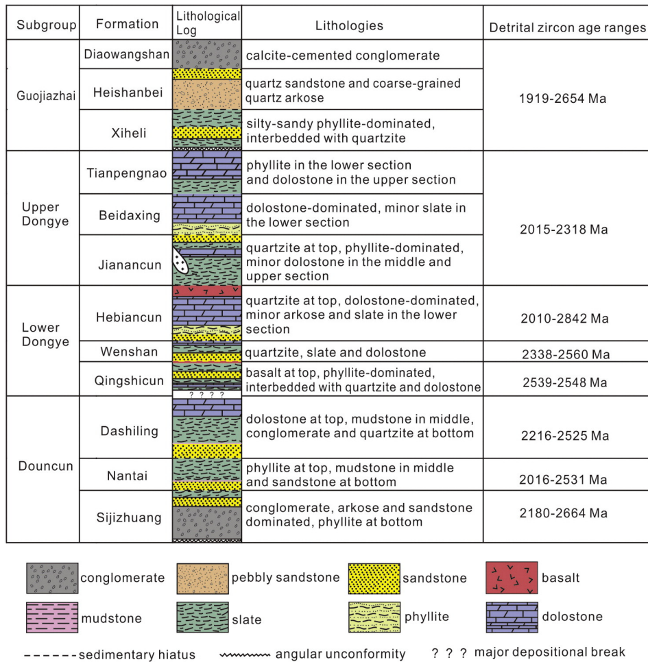
Fig. 23. Stratigraphic section of Hutuo group, with ages of detrital zircons. Modified from Liu et al. (2011b).
