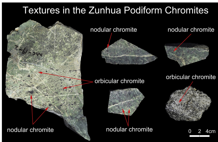
Fig. 11. Photographs of nodular and orbicular textures of podiform chromites (chromites in dunite envelopes cutting harzburgite tectonite) from the Zunhua ophiolitic mélangé. Nodular and orbicular textures in podiform chromites like these illustrated are only known from ophiolites or the modern sea-floor, of any age, anywhere in the world.
