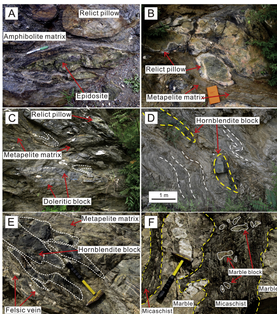
Fig. 6. Field photographs of exotic blocks in the Zhanhuang mélangé. A: Mafic blocks that are interpreted as deformed pillow structures with epidosite lenses preserved in the altered cores, all within an amphibolitic matrix. B: Mafic blocks interpreted as relict pillows dispersed in a metapelite matrix. C: Strongly sheared and disrupted mélangé containing doleritic blocks and relict pillow fragments with epidosite cores in a metapelite matrix. D: Ultramafic blocks in strongly deformed metapelite matrix. E: Ultramafic blocks dispersed in a metapelite matrix. F: Broken-apart marble layer and blocks in strongly deformed matrix of micaschist. Modified from Wang et al., 2013a; Wang et al., 2013b (see Wang et al., 2013a for locations).
