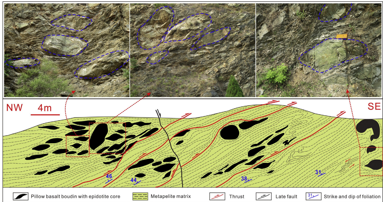
Fig. 5. Structural profile of ophiolitic mélangé in Zanhuang massif. Modified from Wang et al. (2016a, 2016b). Original mapping at 1:200 scale.
