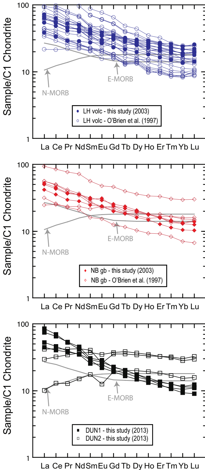
Figure 6. C1-chondrite normalized diagrams of rare earth elements (REE). Normalization values from Sun and McDonough (1989). LH Volc = Lawrence Head Volcanics, NB gb = gabbro sills from the New Bay Formation, DUN1 and DUN2 = blocks from the Dunnage Mélange. Year listed for this study (2003, and/or 2013) refers to the analysis date of each suite of samples.
