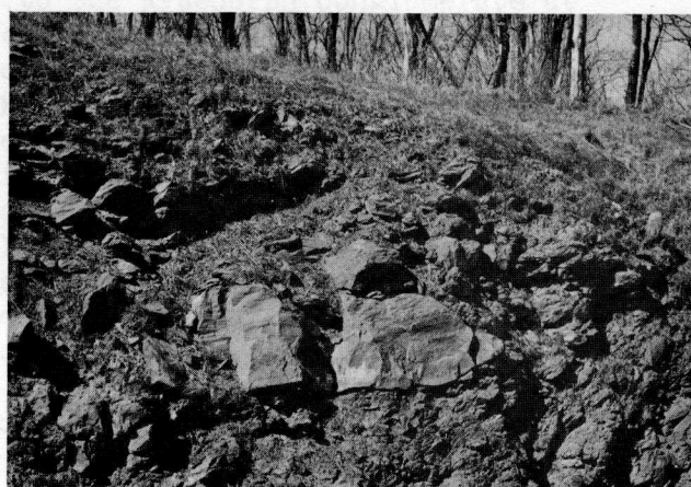
F. Wildflysch-like conglomerate of blocks of limestone, quartzite and the greywacke of the Austin Glen Member, in Normanskill Shale. Road cut on Route 151, two miles east of Rensselaer, New York.
