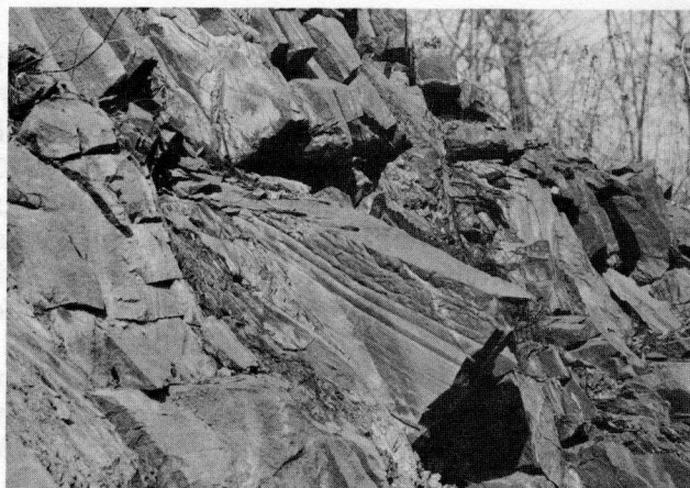
B. Groove casts, some with superimposed load casts.
