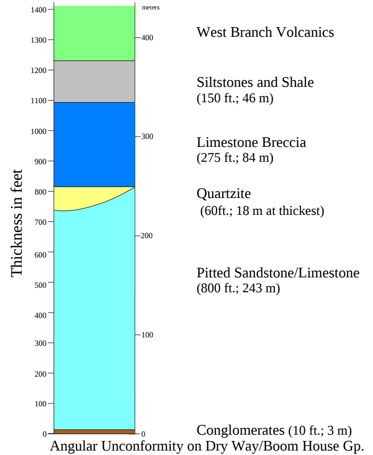
Stratigraphic Column of the Ripogenus Formation
