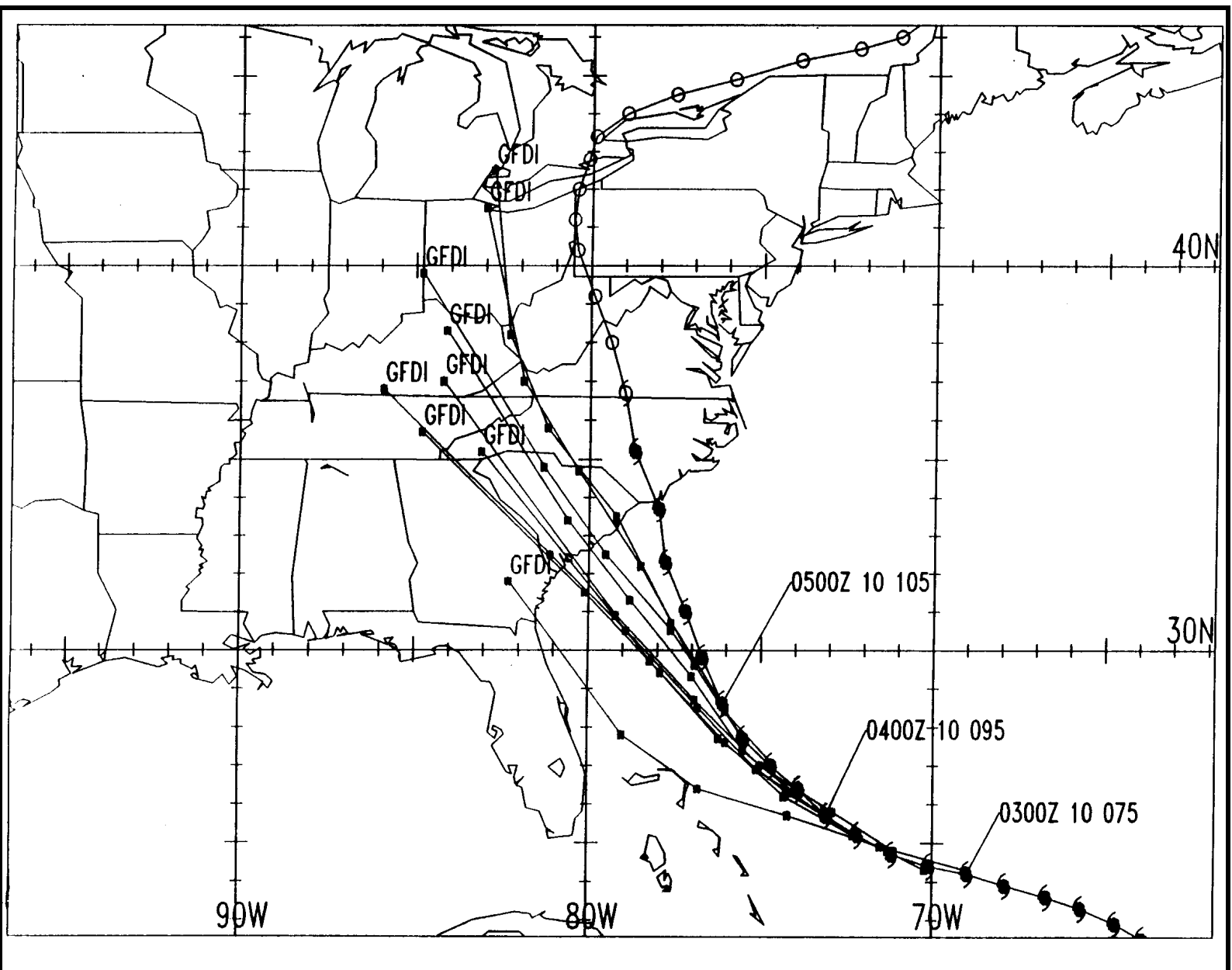
Figure 5: GFDL guidance on Hurricane Fran from 8 p.m. September 2 (0000 Coordinated Universal Time [UTC] September 3) to 8 p.m. September 4 (0000 UTC September 5), showing a left bias.
