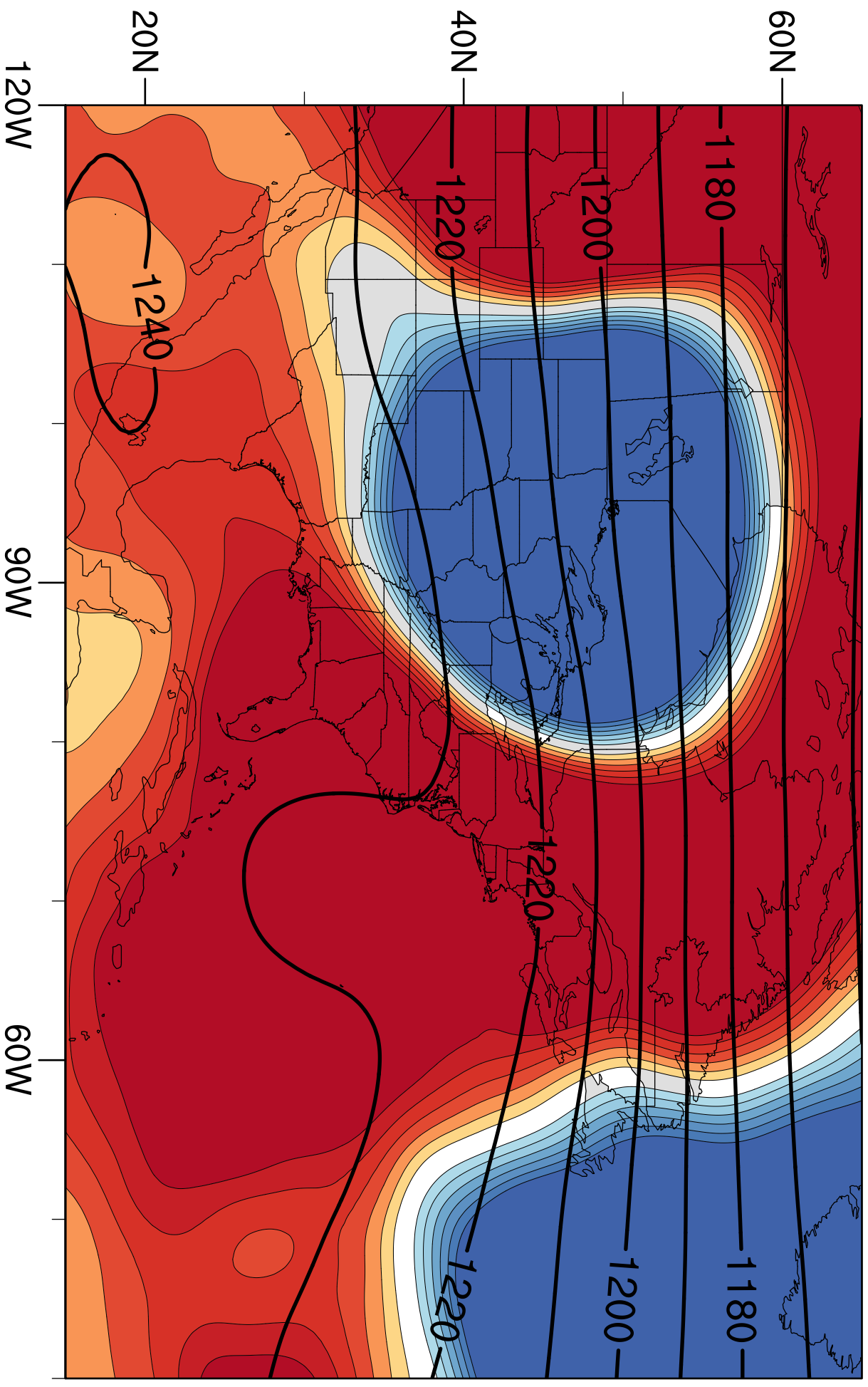
(f) EOF 6: 2.3%
