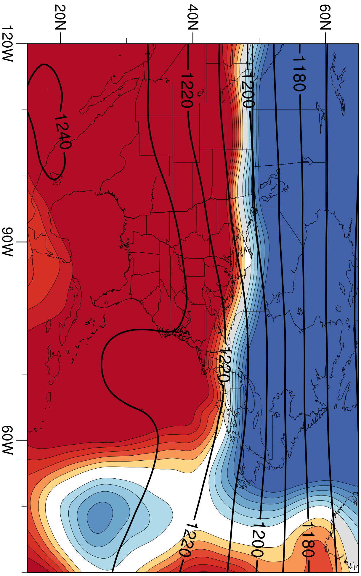
(e) EOF 5: 2.9%
