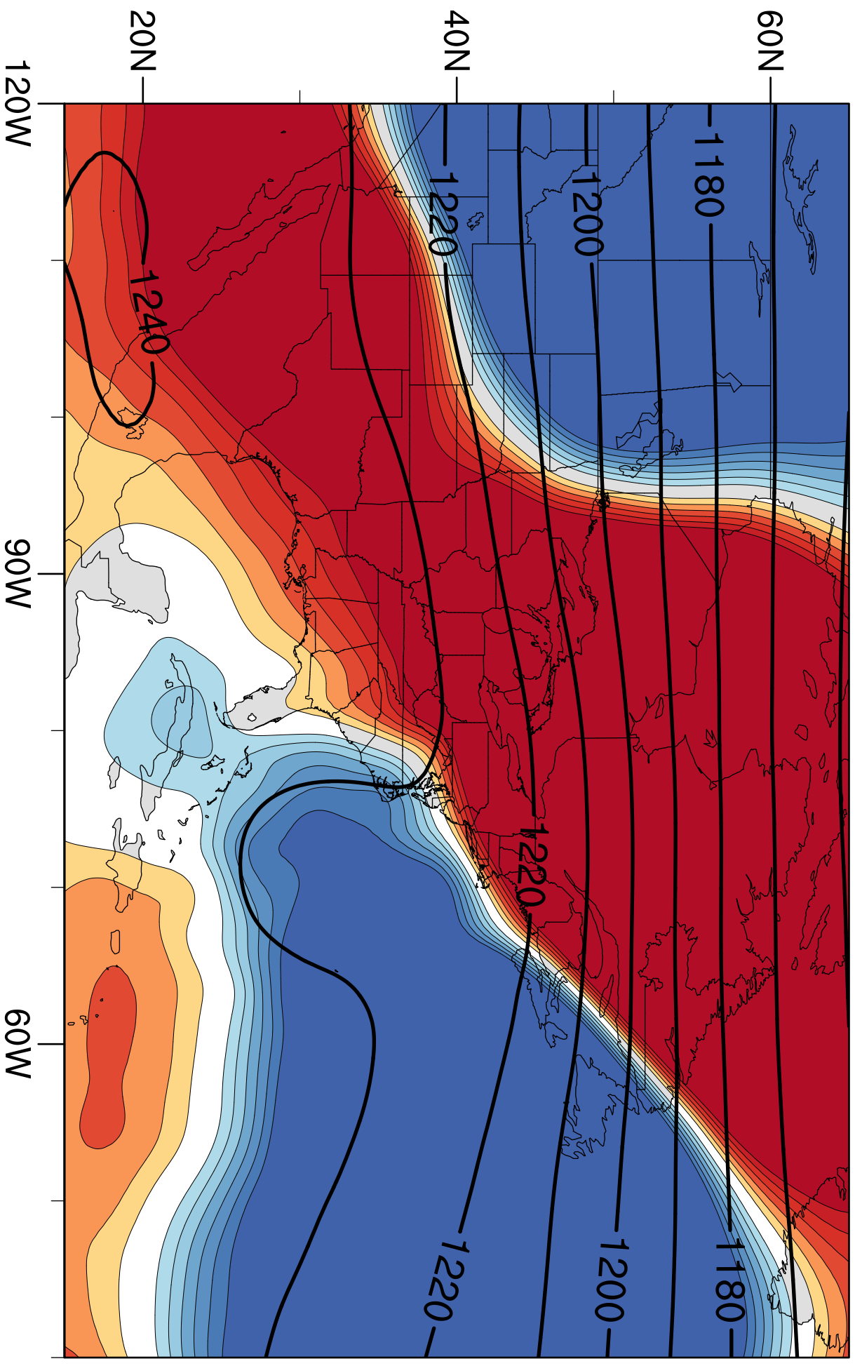
(c) EOF 3: 5.6%
