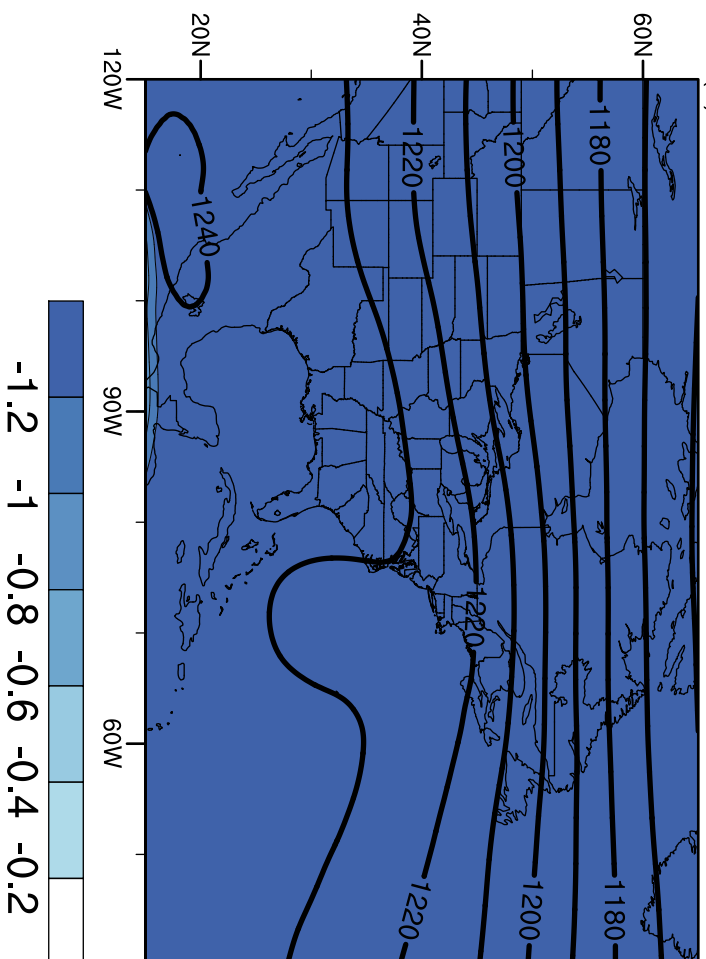
(a) EOF 1: 69.6%
