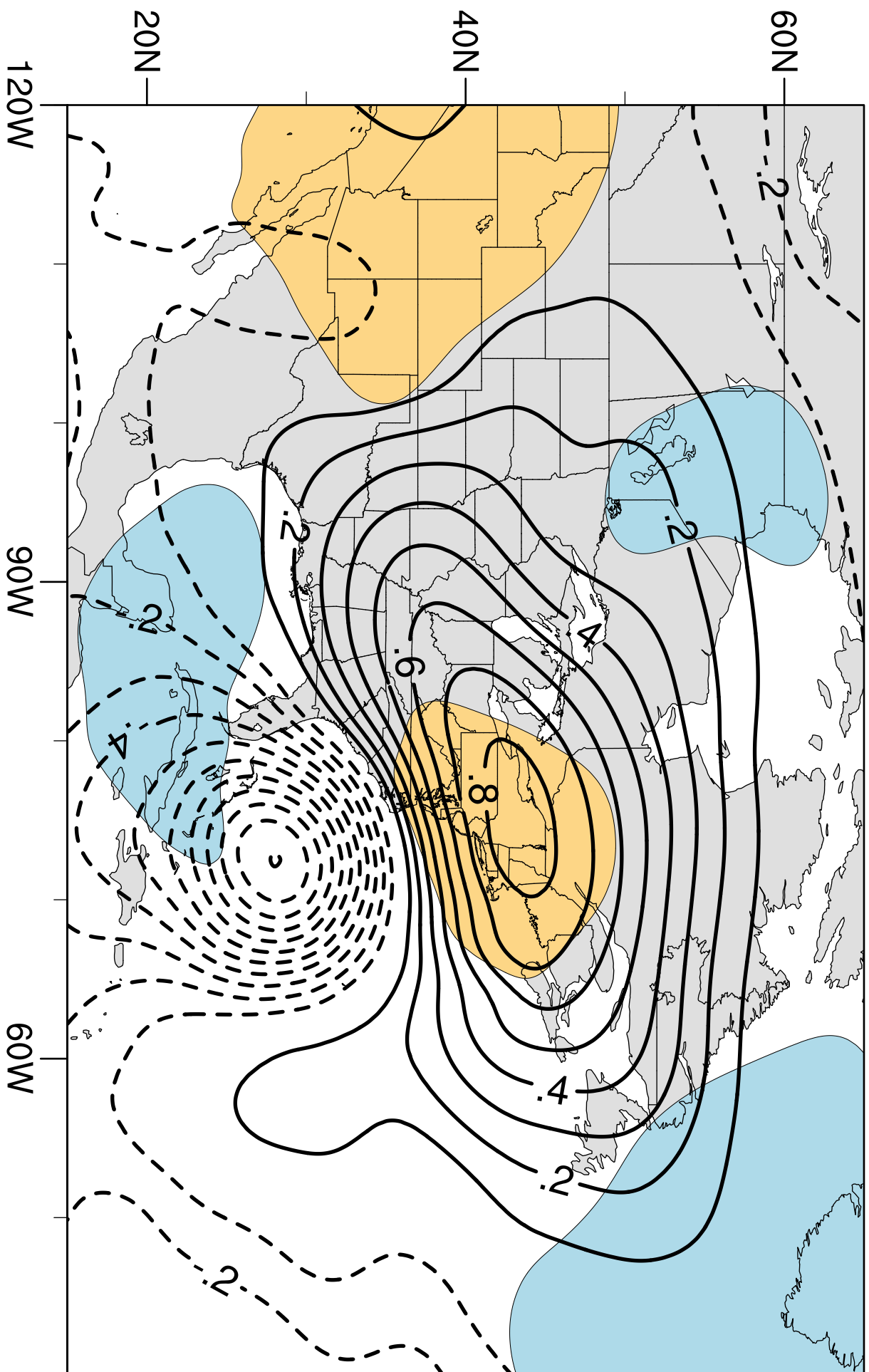
(g) EOF 7: 4.2%
