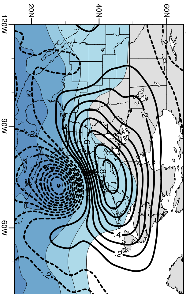
(a) EOF 1: 30.6%
