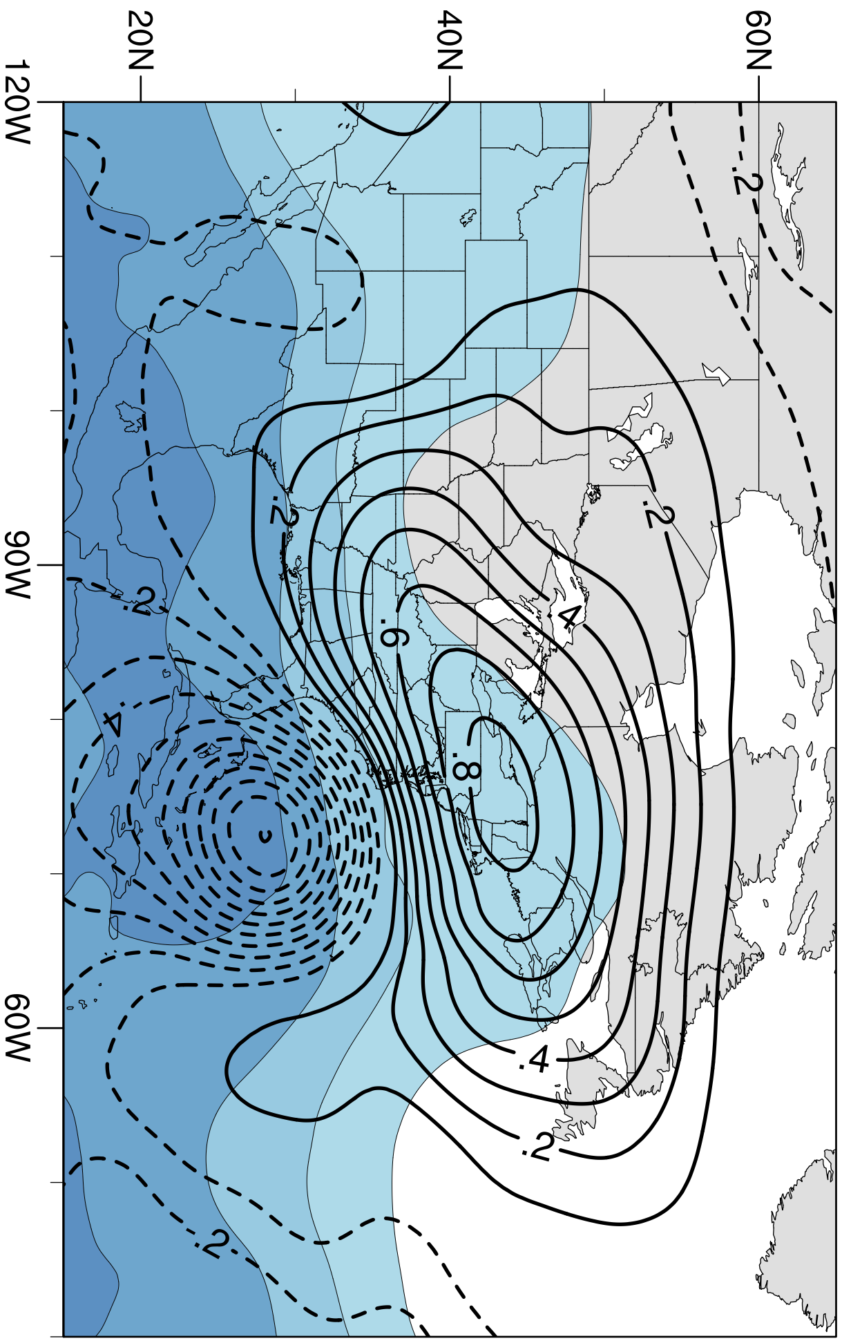
(a) EOF 1: 30.6%
