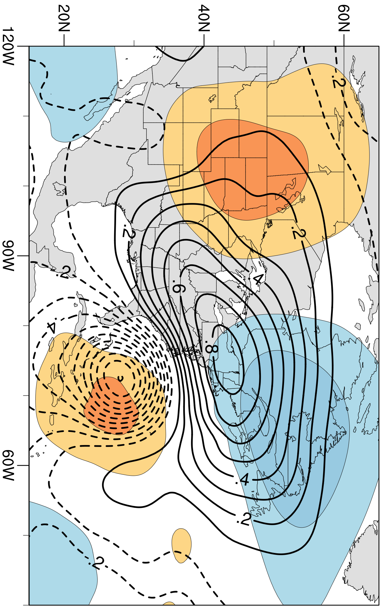
(c) EOF 3: 9.6%
