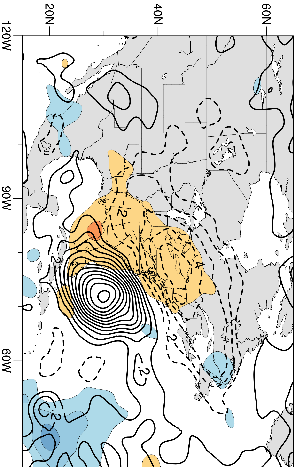
(f) EOF 6: 4.7%
