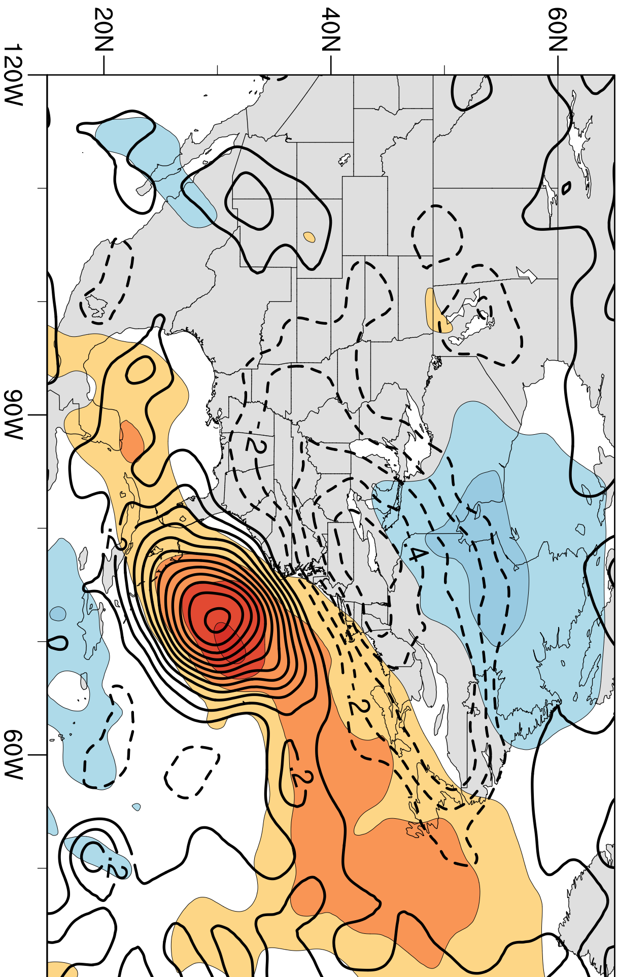
(a) EOF 1: 10.2%
