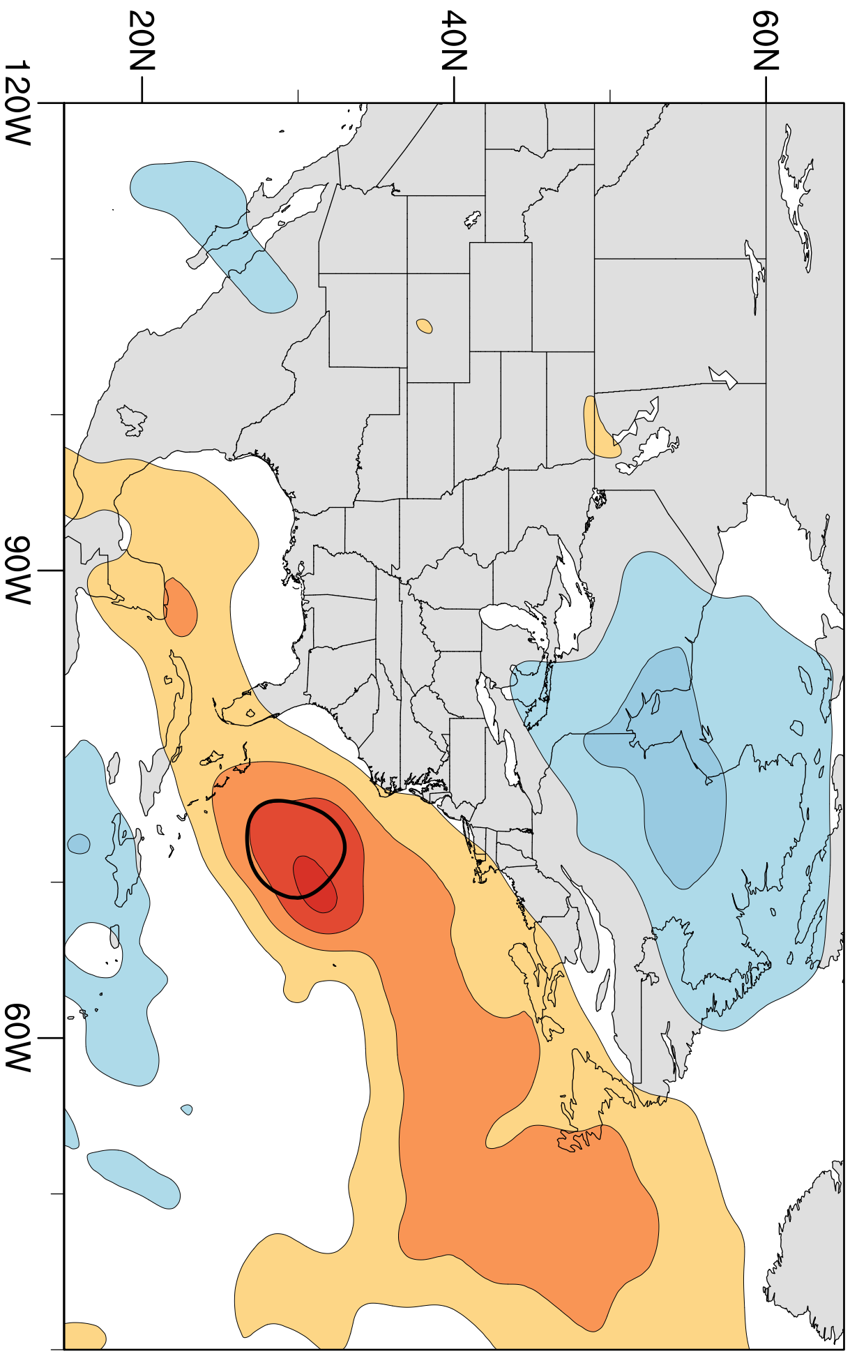
(a) EOF 1: 10.2%
