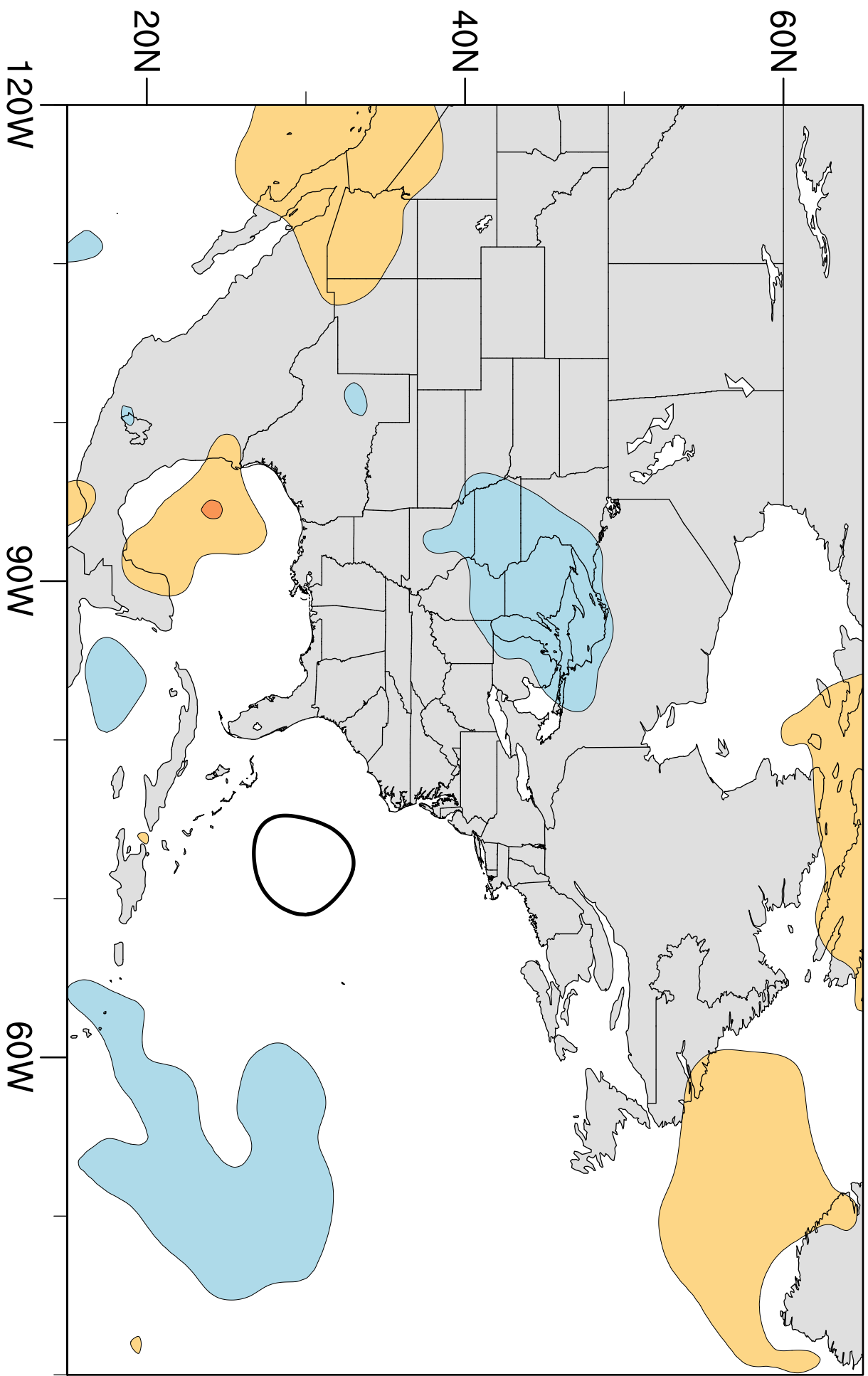
(g) EOF 7: 3.7%
