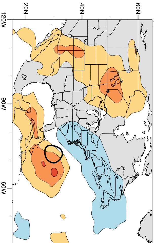
(b) EOF 2: 8.9%
