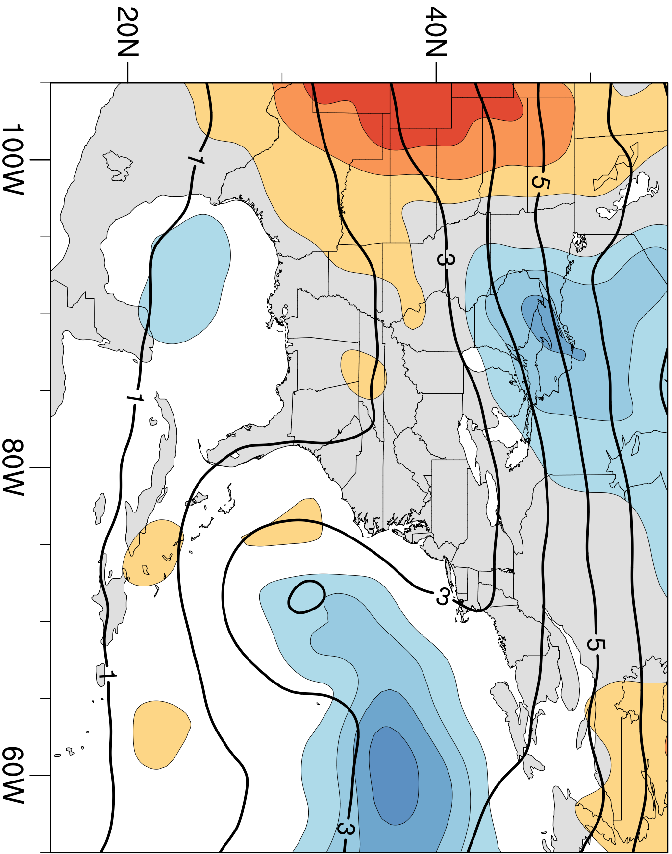
(f) EOF 6: 3.8%
