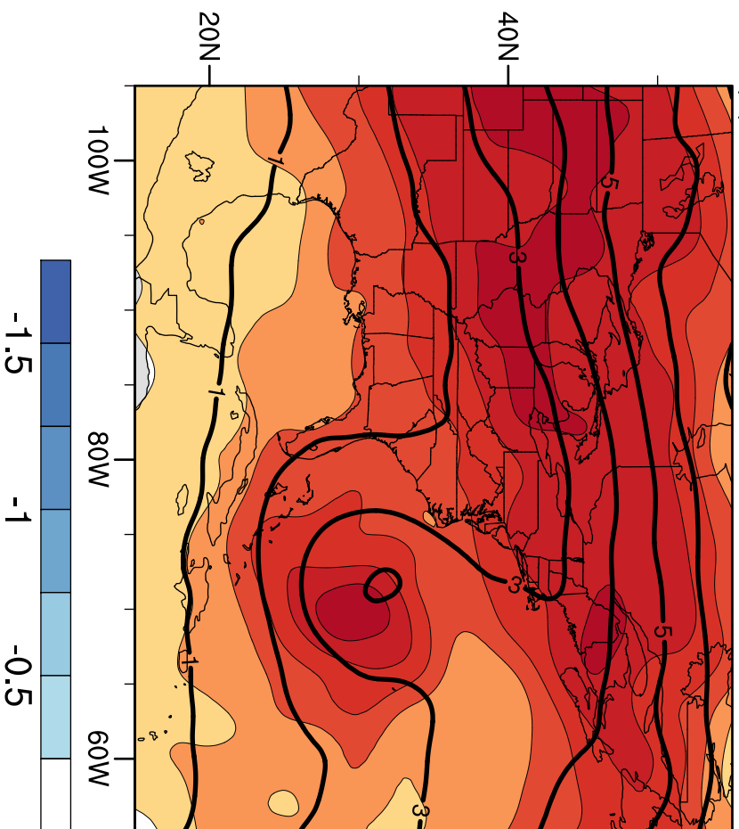
(a) EOF 1: 34.3%
