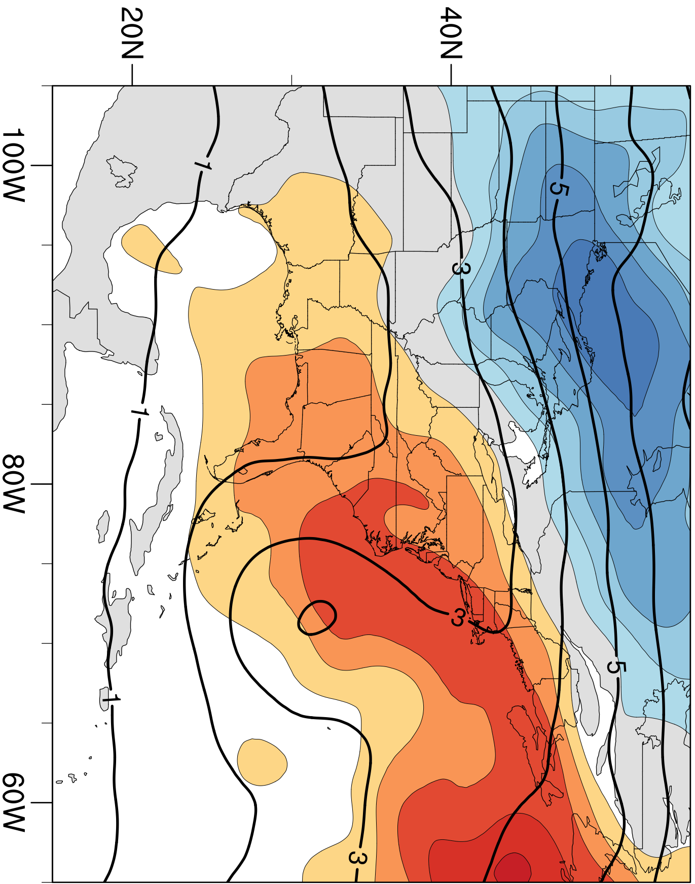
(c) EOF 3: 10.3%
