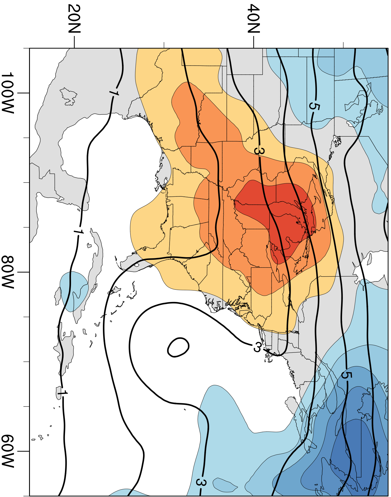
(e) EOF 5: 6%
