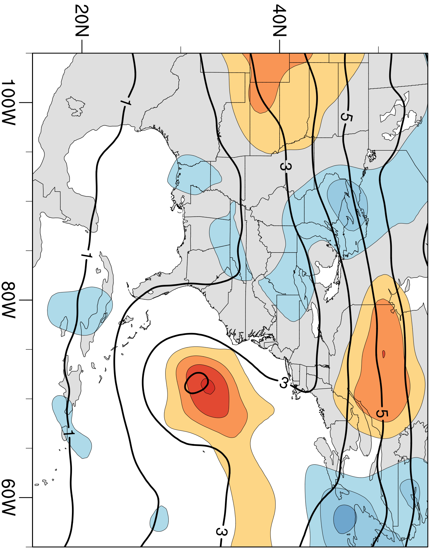
(h) EOF 8: 2.6%
