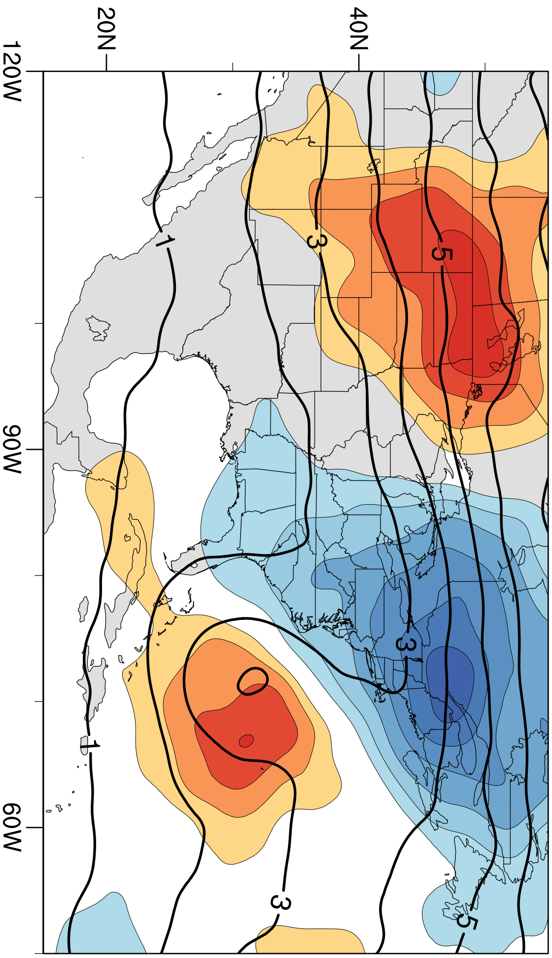
(c) EOF 3: 8.4%
