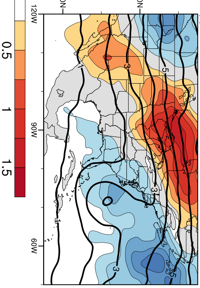
(b) EOF 2: 9.2%
