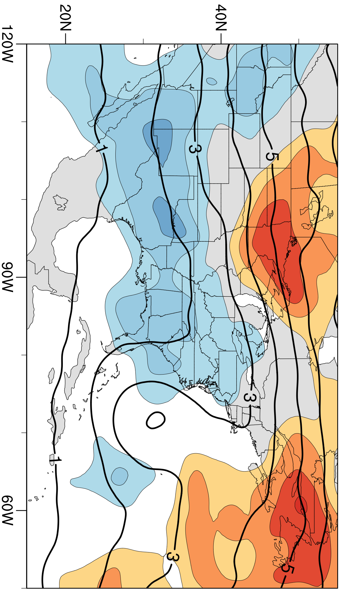
(e) EOF 5: 5.5%
