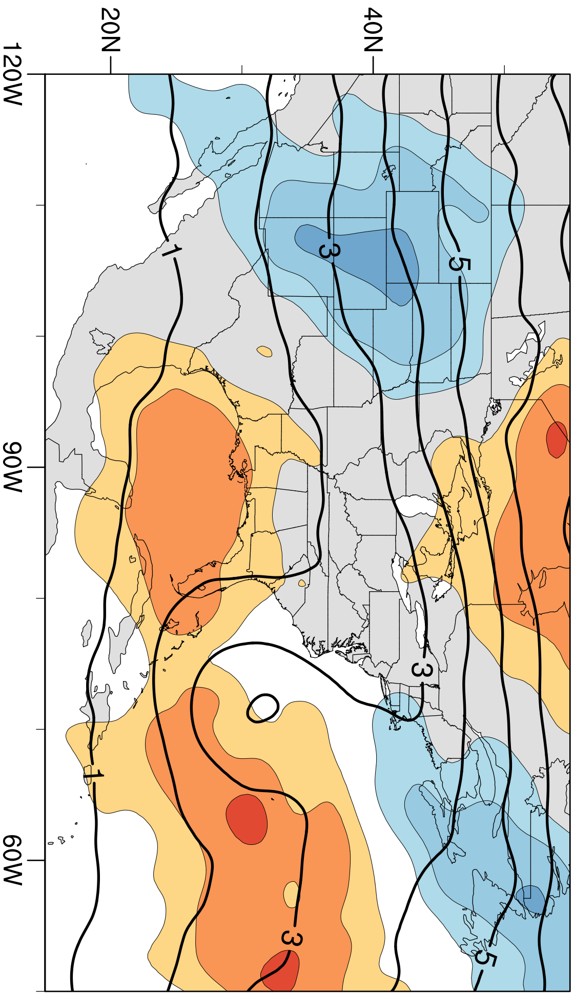
(f) EOF 6: 4.8%
