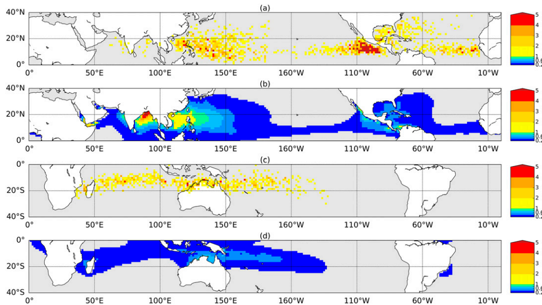
FIG. 13. Global spatial distribution of (a) TC genesis points in boreal summer (JJAS), (b) tropical cyclone genesis index (TCGI) density in boreal summer (JJAS), (c) TC genesis points in austral summer (DJFM), and (d) TCGI density in austral summer (DJFM). Each grid point represents the number of storms that occur over 34 years in the given 4-month season.
