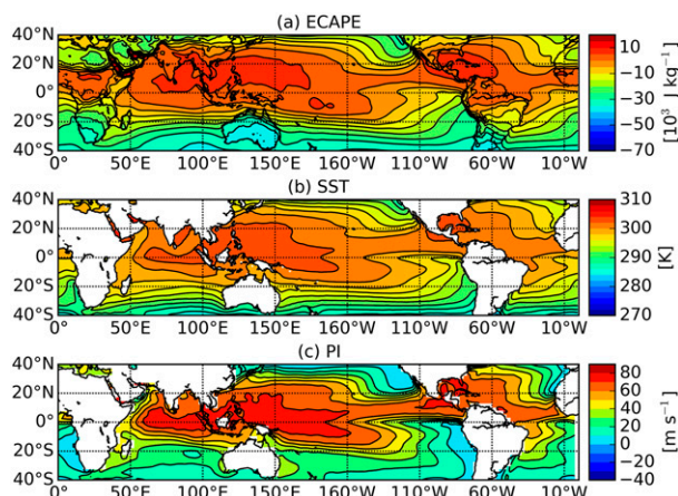
FIG. 3. JJAS climatologies of (a) estimated convective available potential energy (ECAPE, 10^3 \text{ J kg}^{-1} ), (b) sea surface temperature (SST, K), and (c) potential intensity expressed in wind speed (PI, \text{m s}^{-1} ). Note the spatial similarities that exist across all three variables.
