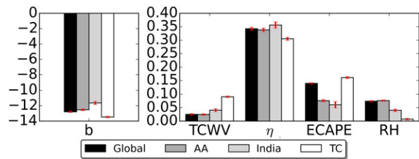
FIG. 12. Statistics from Poisson regressions between monsoon disturbance genesis points and mean state environmental variables over the entire globe, the Asian–Australian region, the Indian continent region, and between TC genesis points and the same mean state environmental variables over the entire globe. Red error bars indicate bootstrap errors.
